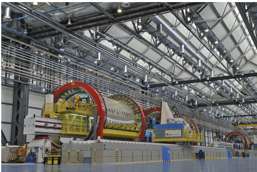
Fueselage section of B-787 in AFP Technology
